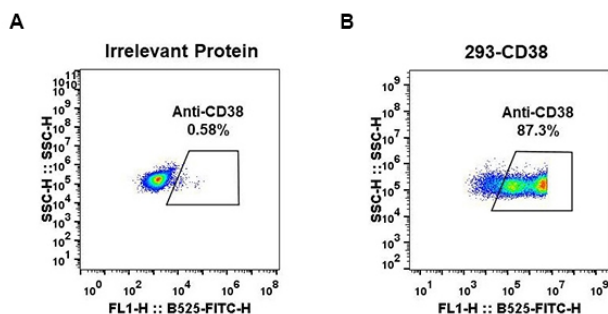
Figure 1. Expi 293 cell line transfected with irrelevant protein (left) and human CD38 (right) were surface stained with Rabbit anti-CD38 monoclonal antibody 1µg/ml (clone: DM28) followed by Alexa 488-conjugated anti-rabbit IgG secondary antibody.
