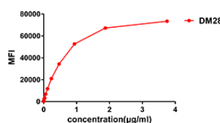
Figure 2. Flow cytometry data of serially titrated Rabbit anti-CD38 monoclonal antibody (clone: DM28) on Raji cells. The Y-axis represents the mean fluorescence intensity (MFI) while the X-axis represents the concentration of IgG used.
