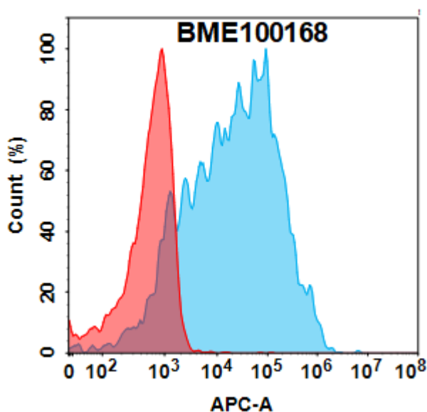
Figure 1. Flow cytometry analysis with 1µg/mL Anti-CD70 (Chongqing Precision biosimilar) mAb (28159) on Expi293 cells transfected with Human CD70 protein (Blue histogram) or Expi293 transfected with irrelevant protein (Red histogram).
