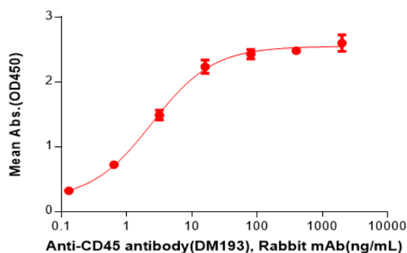
Figure 2. ELISA plate pre-coated by 2 µg/ml (100 µl/well) Human CD45 Protein, His Tag(11380) can bind Anti-CD45 antibody(DM193), Rabbit mAb in a linear range of 0.64-16.00 ng/mL.
