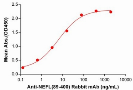
Figure 2. ELISA plate pre-coated by 1 \mu g/ml (100 \mu l/well) Human NEFL (89-400) Protein, His Tag (11444) can bind Anti-NEFL(89-400) antibody(DM199), Rabbit mAb 28542 in a linear range of 0.128-80 ng/mL.
