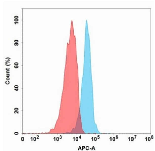
Figure 2. Flow cytometry analysis with 15 \mu\text{g}/\text{mL} Anti-ITGA4 (natalizumab) mAb (28077) on Expi293 cells transfected with Human ITGA4 protein (Blue histogram) or Expi293 transfected with irrelevant protein (Red histogram).
