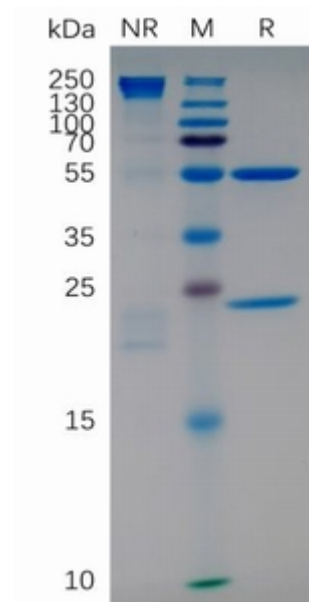
Figure 1. Anti-ITGA4 (natalizumab biosimilar) mAb on SDS-PAGE under non-reducing (NR) and reducing (R) conditions.
