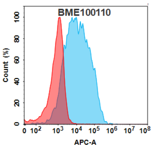
Figure 1. Flow cytometry analysis with 15µg/mL Anti-TLR2(tomaralimab biosimilar) mAb (28109) on Expi293 cells transfected with Human TLR2 protein (Blue histogram) or Expi293 transfected with irrelevant protein (Red histogram).
