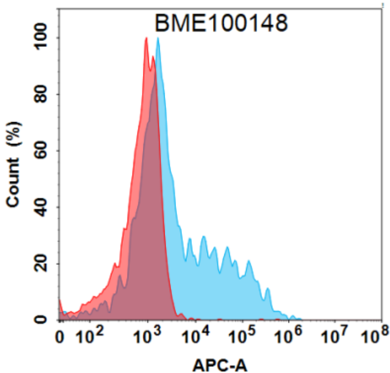
Figure 1. Flow cytometry analysis with 15 \mu\text{g}/\text{mL} Anti-OSMR (vixarelimab biosimilar) mAb (28140) on Expi293 cells transfected with Human OSMR protein (Blue histogram) or Expi293 transfected with irrelevant protein (Red histogram).
